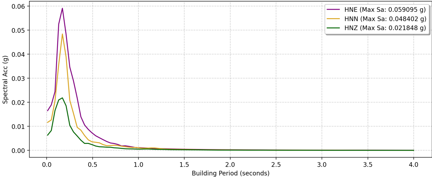
Response Spectrum Overlay (N, E, Z) - Stasiun PRJI
