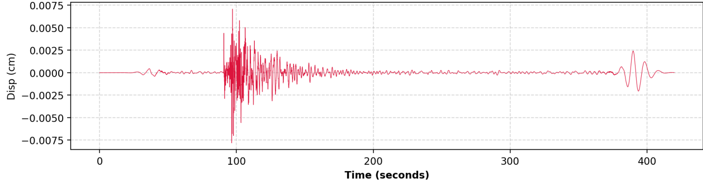
4. Displacement (HNZ | PGD: 0.007833 cm)
