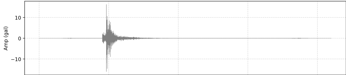
2. Filtered Acceleration (HNE | PGA: 0.162402 m/s 2 )
