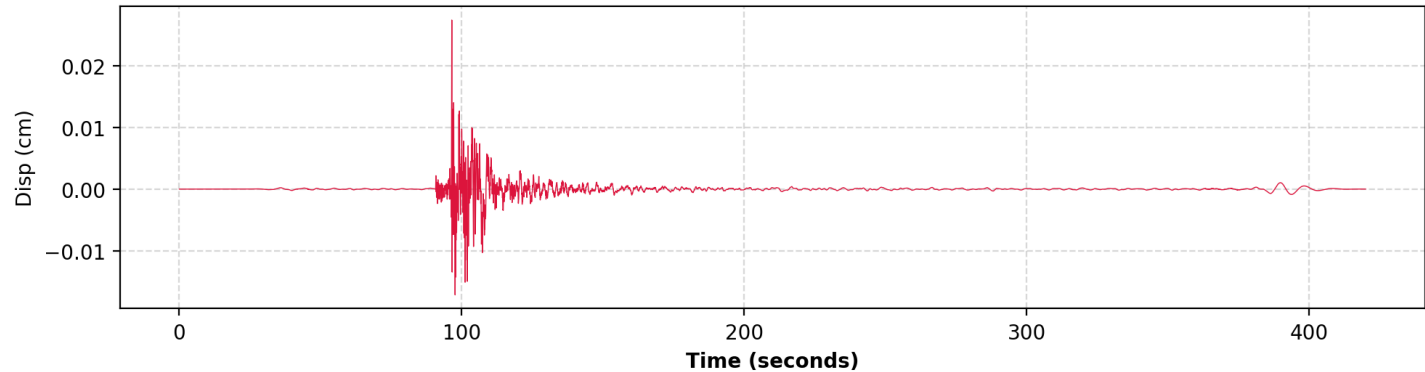
4. Displacement (HNE | PGD: 0.027479 cm)
