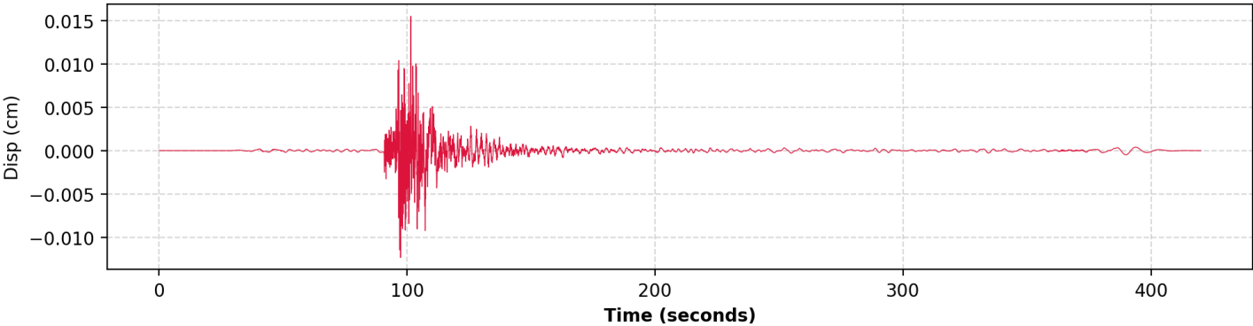
4. Displacement (HNN | PGD: 0.015495 cm)
