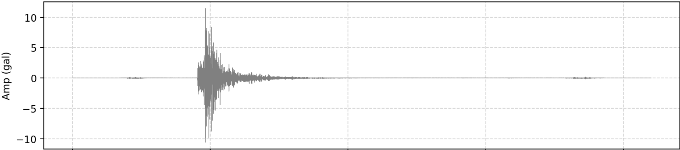
2. Filtered Acceleration (HNN | PGA: 0.114586 m/s 2 )
