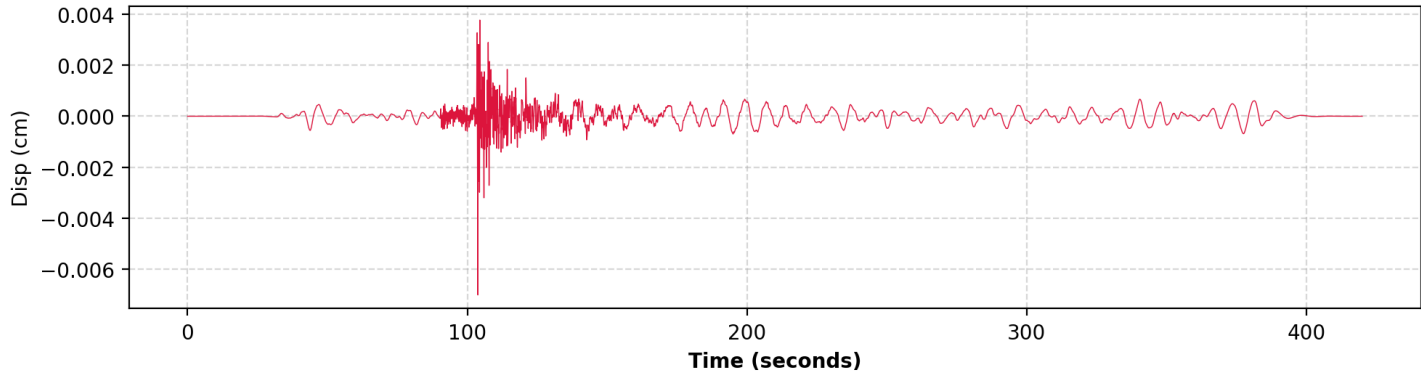
4. Displacement (HNE | PGD: 0.007004 cm)
