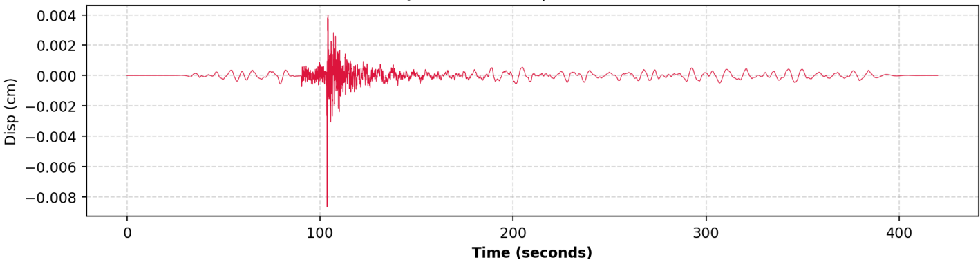
4. Displacement (HNN | PGD: 0.008664 cm)
