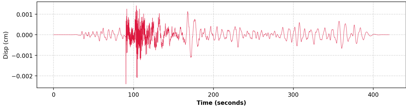
4. Displacement (HNZ | PGD: 0.002399 cm)
