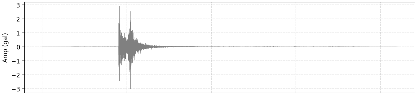
2. Filtered Acceleration (HNZ | PGA: 0.030075 m/s 2 )
