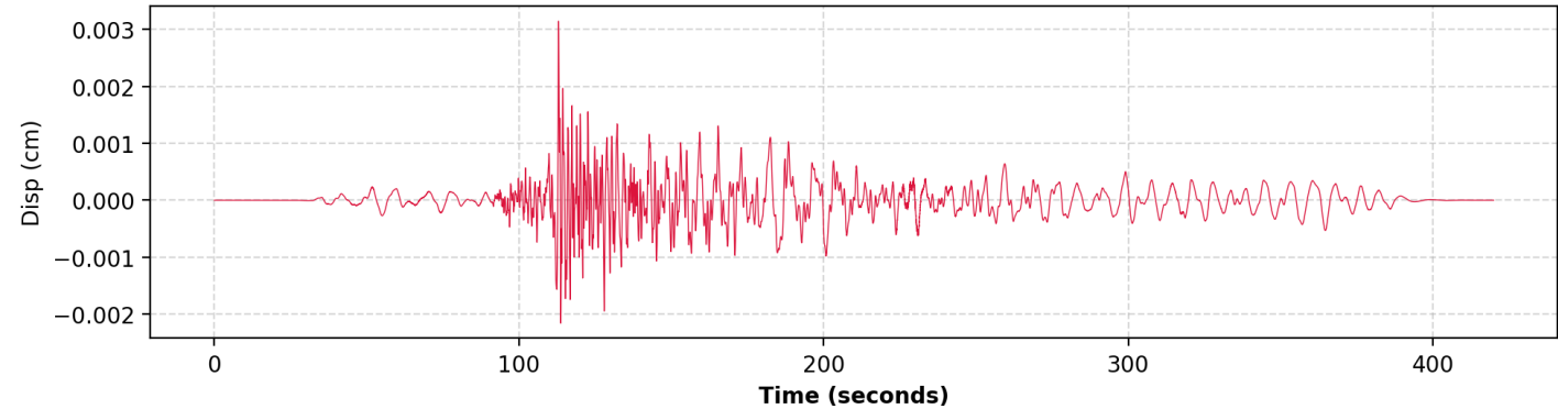
4. Displacement (HNN | PGD: 0.003147 cm)
