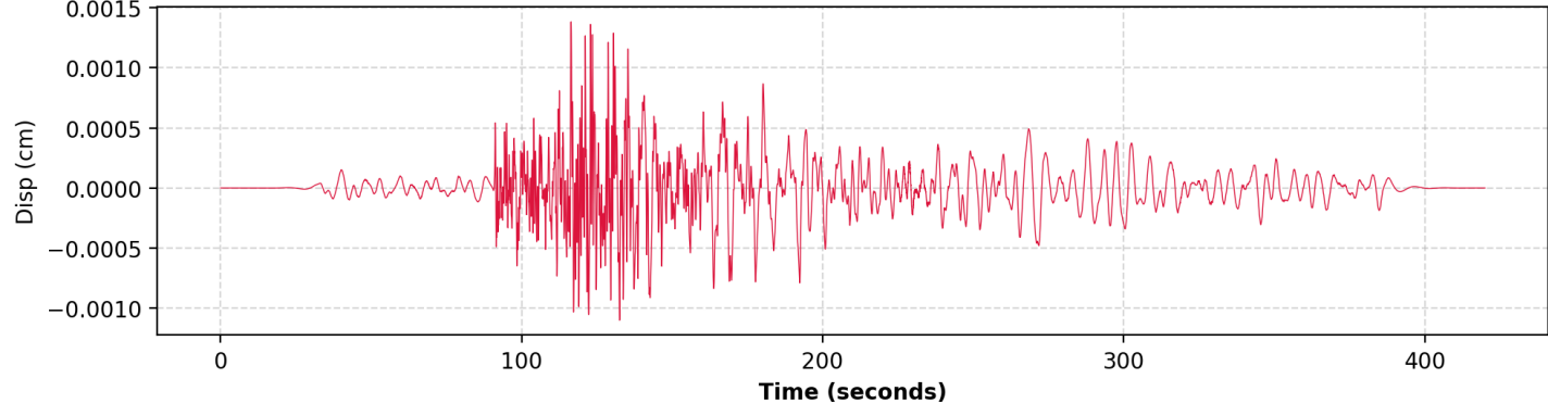
4. Displacement (HNZ | PGD: 0.001383 cm)
