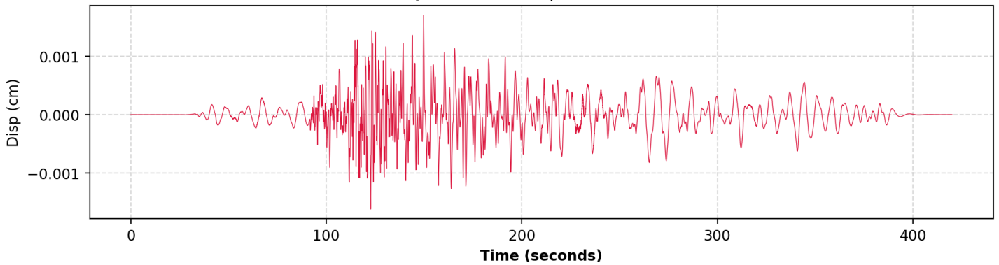
4. Displacement (HNE | PGD: 0.001699 cm)
