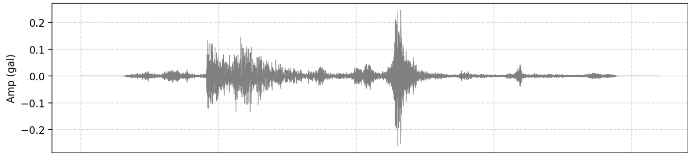
2. Filtered Acceleration (HNZ | PGA: 0.002614 m/s 2 )
