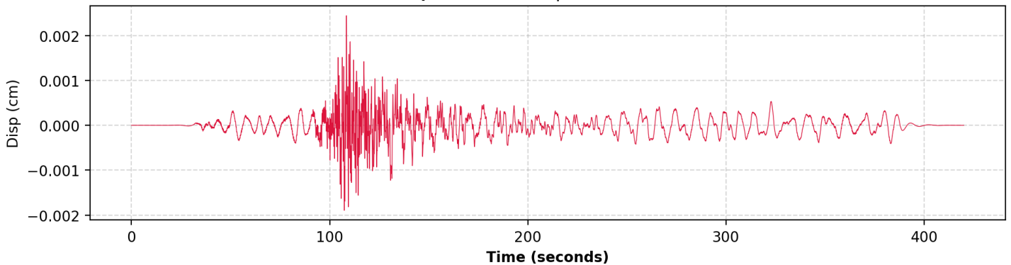
4. Displacement (HNE | PGD: 0.002443 cm)
