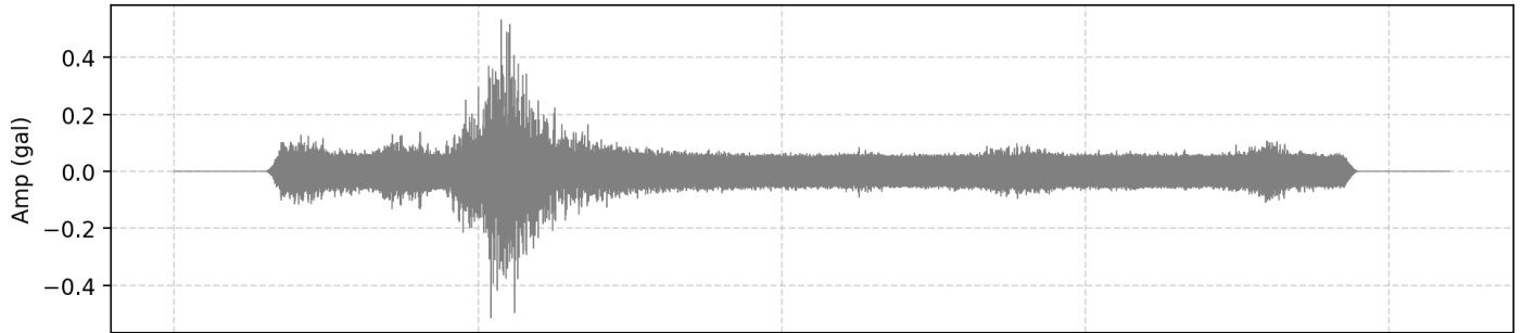
2. Filtered Acceleration (HNE | PGA: 0.005325 m/s 2 )
