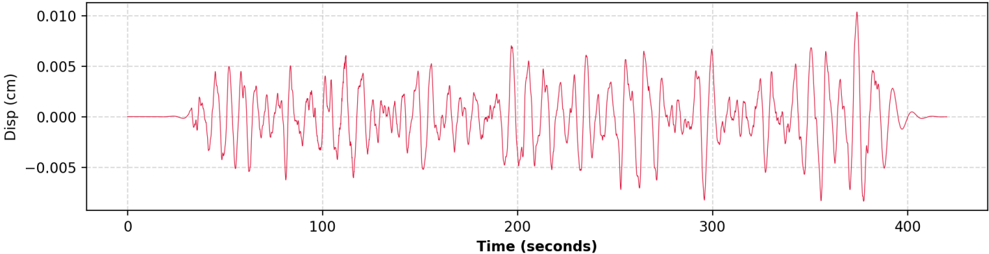
4. Displacement (HNN | PGD: 0.010366 cm)
