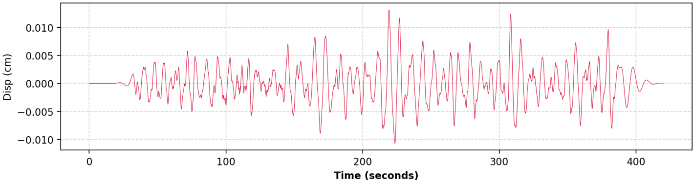
4. Displacement (HNE | PGD: 0.013126 cm)
