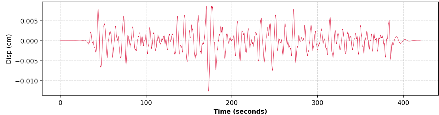
4. Displacement (HNZ | PGD: 0.012631 cm)
