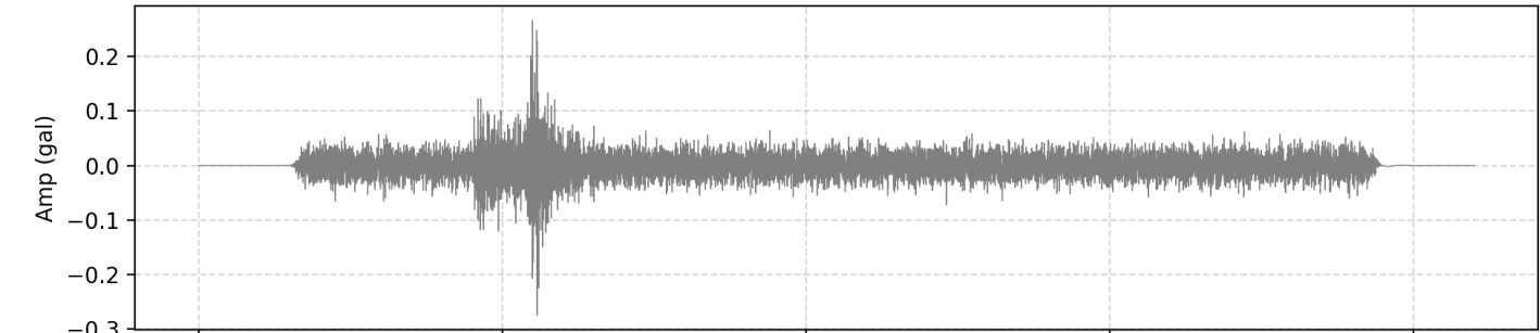
2. Filtered Acceleration (HNN | PGA: 0.002748 m/s 2 )
