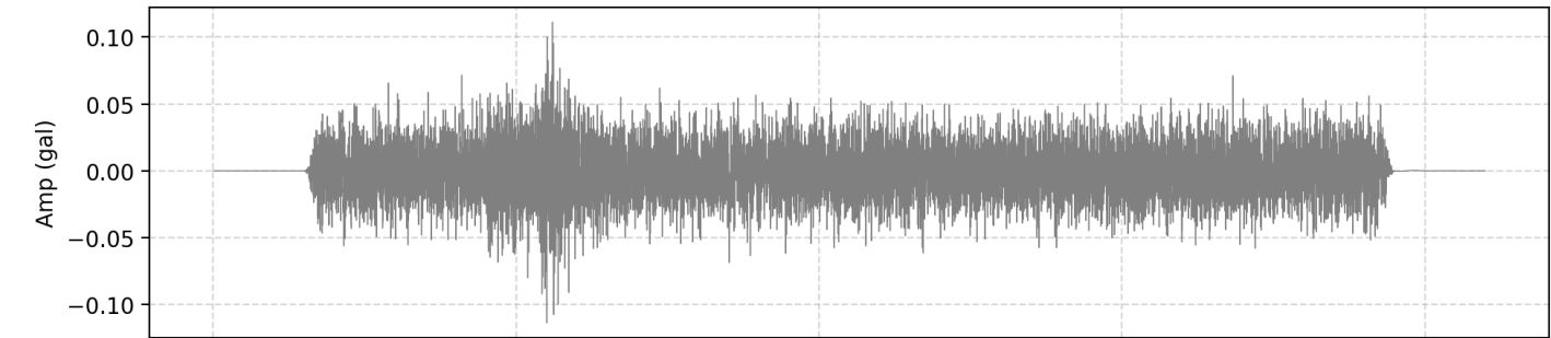
2. Filtered Acceleration (HNZ | PGA: 0.001136 m/s 2 )
