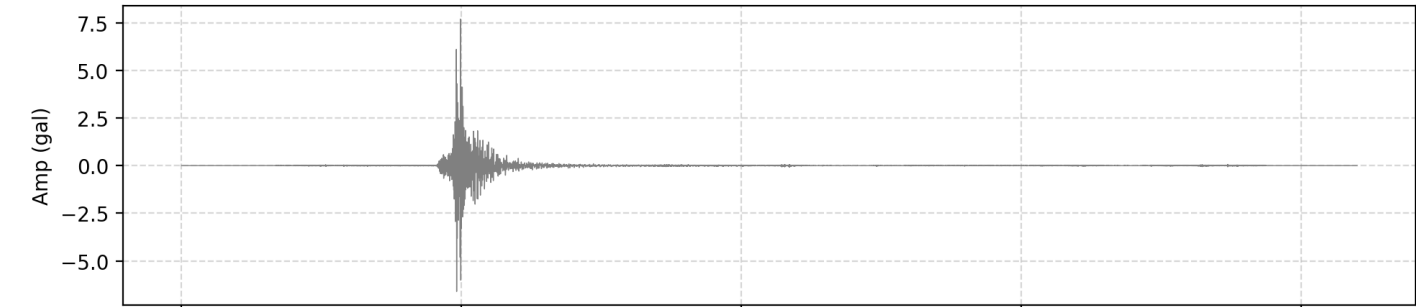
2. Filtered Acceleration (HNN | PGA: 0.076860 m/s 2 )
