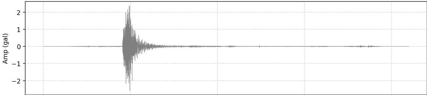
2. Filtered Acceleration (HNZ | PGA: 0.025836 m/s 2 )
