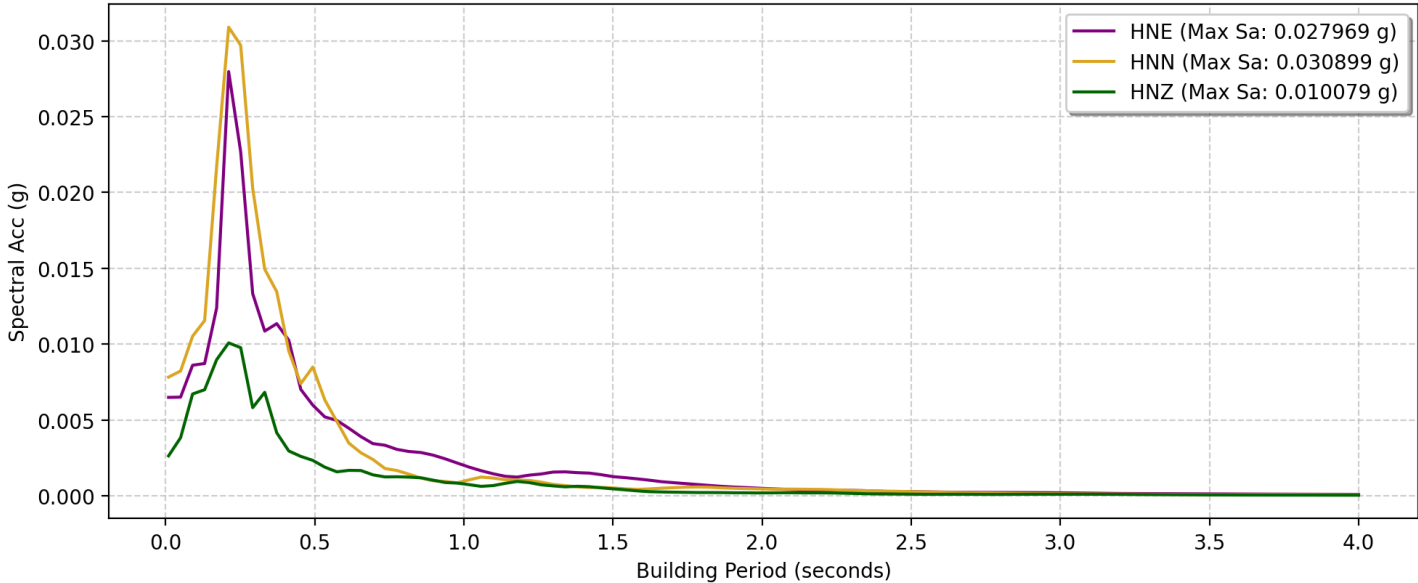
Response Spectrum Overlay (N, E, Z) - Stasiun BOJI
