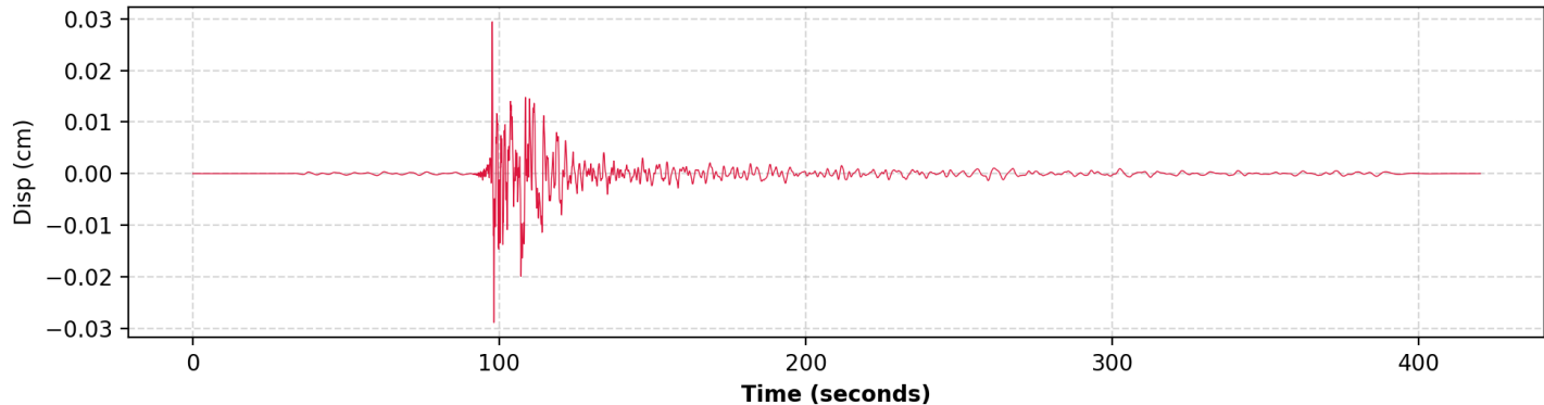
4. Displacement (HNE | PGD: 0.029414 cm)
