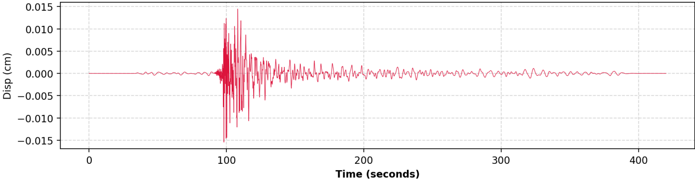
4. Displacement (HNN | PGD: 0.015428 cm)
