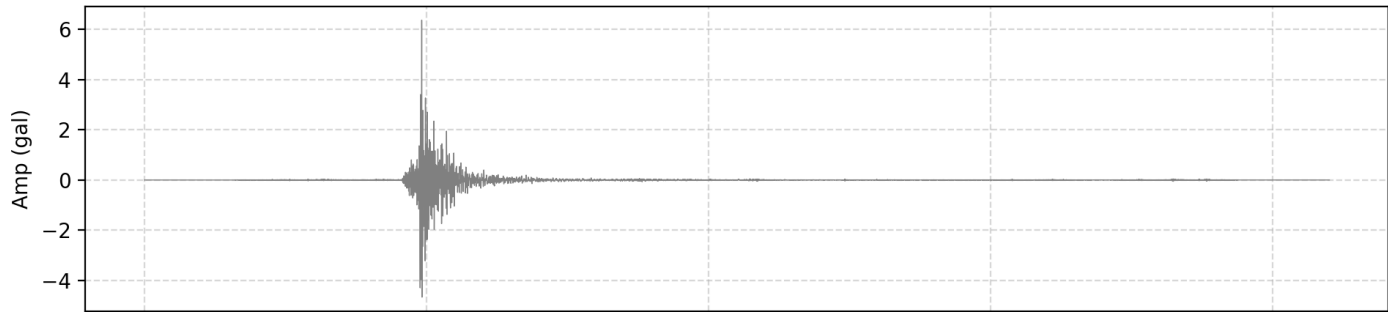
2. Filtered Acceleration (HNE | PGA: 0.063697 m/s 2 )
