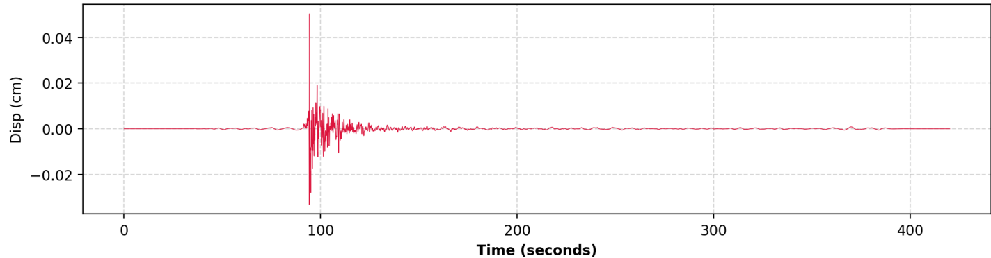
4. Displacement (HNN | PGD: 0.050260 cm)
