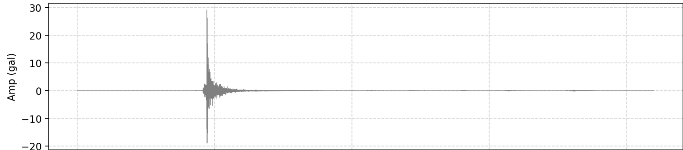
2. Filtered Acceleration (HNN | PGA: 0.291675 m/s 2 )
