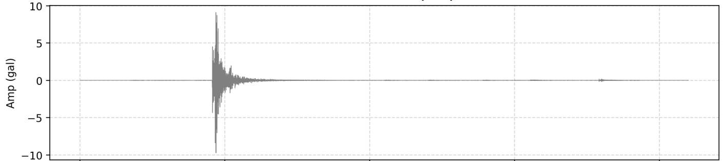
2. Filtered Acceleration (HNZ | PGA: 0.097268 m/s 2 )
