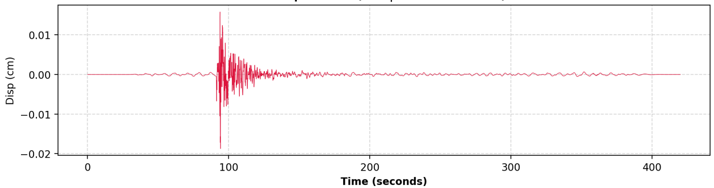
4. Displacement (HNZ | PGD: 0.018744 cm)
