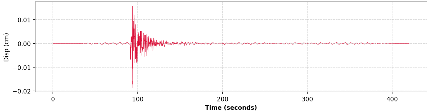
4. Displacement (HNZ | PGD: 0.018744 cm)
