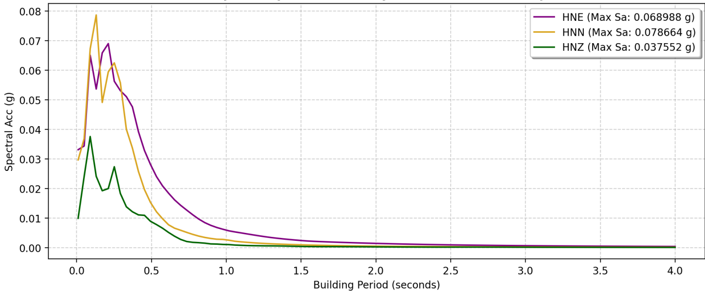
Response Spectrum Overlay (N, E, Z) - Stasiun WGJR
