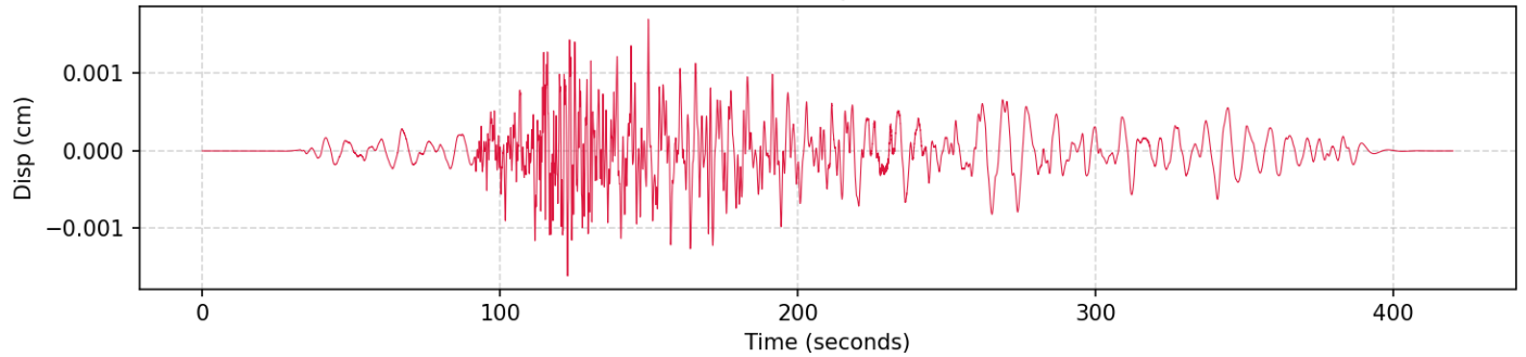
4. Displacement (HNE | PGD: 0.001699 cm)
