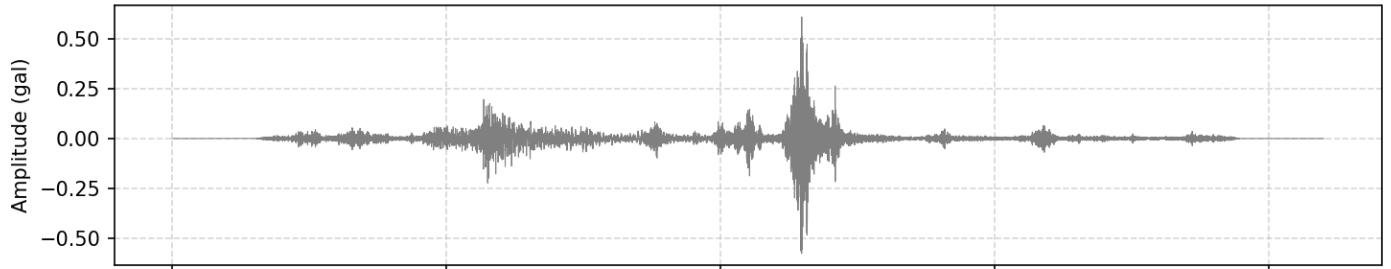
2. Filtered Acceleration (HNE | PGA: 0.006101 m/s 2 )
