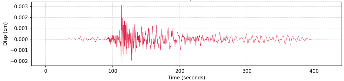
4. Displacement (HNN | PGD: 0.003147 cm)
