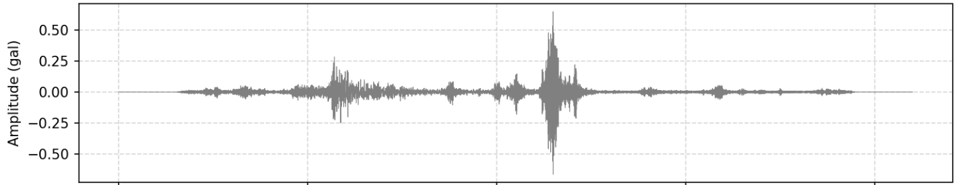
2. Filtered Acceleration (HNN | PGA: 0.006634 m/s 2 )
