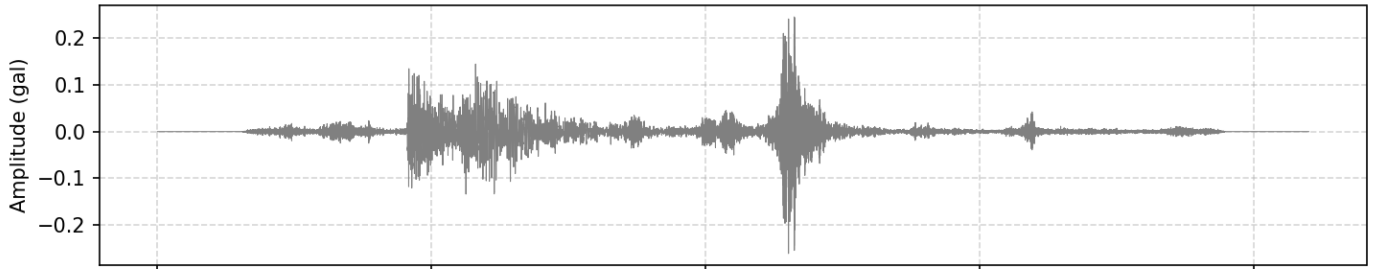
2. Filtered Acceleration (HNZ | PGA: 0.002614 m/s 2 )
