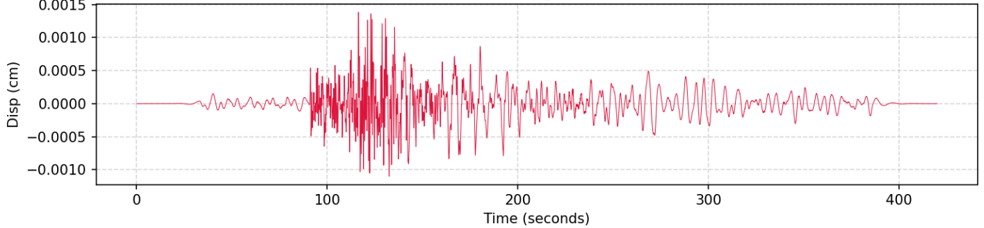
4. Displacement (HNZ | PGD: 0.001383 cm)
