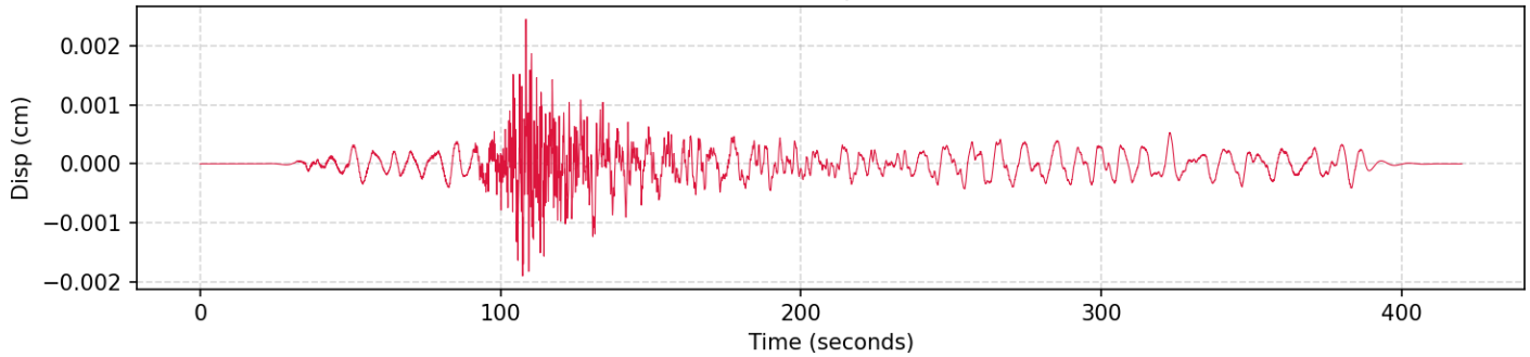
4. Displacement (HNE | PGD: 0.002443 cm)
