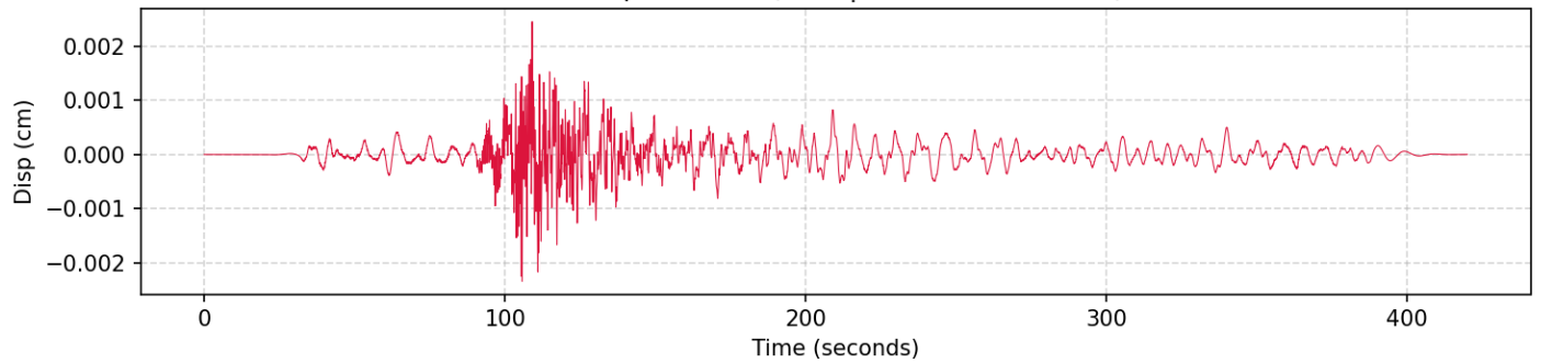
4. Displacement (HNN | PGD: 0.002449 cm)
