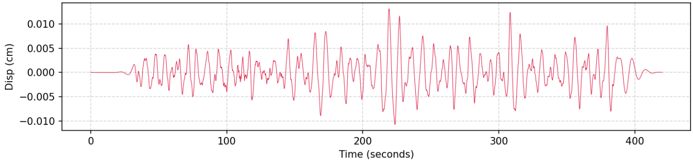
4. Displacement (HNE | PGD: 0.013126 cm)
