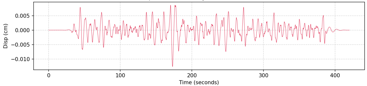
4. Displacement (HNZ | PGD: 0.012631 cm)
