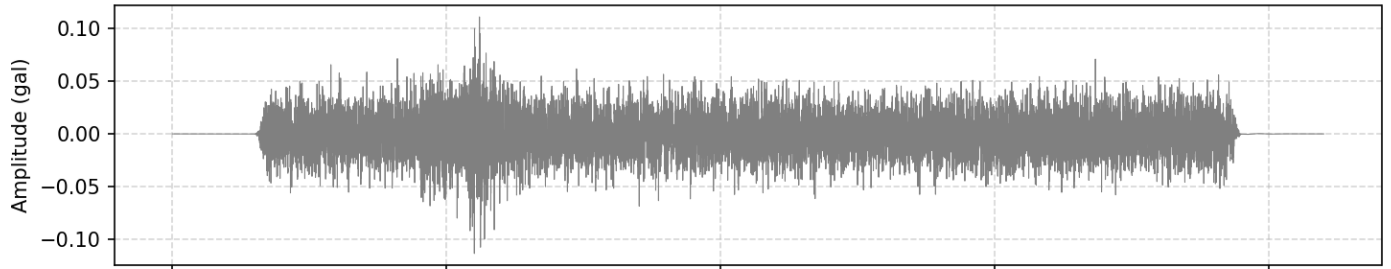
2. Filtered Acceleration (HNZ | PGA: 0.001136 m/s 2 )
