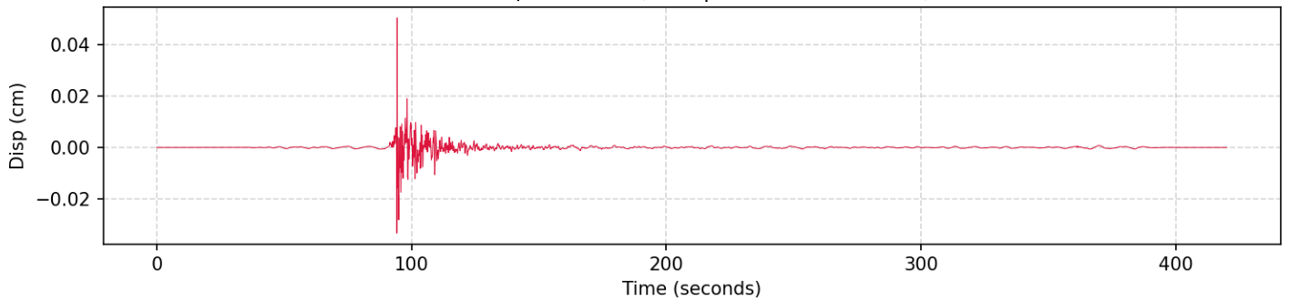
4. Displacement (HNN | PGD: 0.050260 cm)
