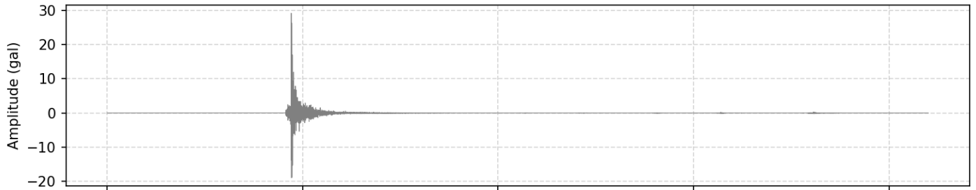
2. Filtered Acceleration (HNN | PGA: 0.291675 m/s 2 )
