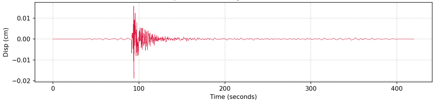
4. Displacement (HNZ | PGD: 0.018744 cm)
