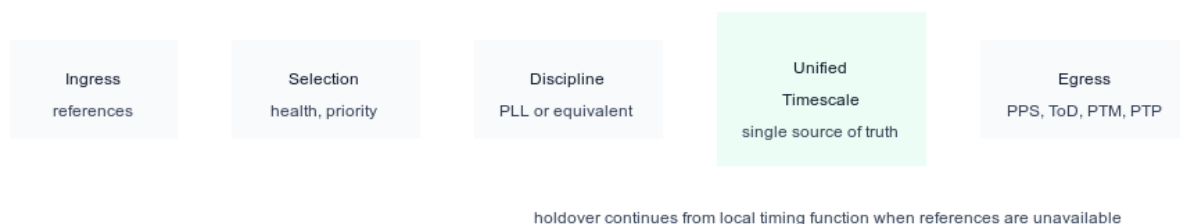
Figure 2: Unified timescale flow
