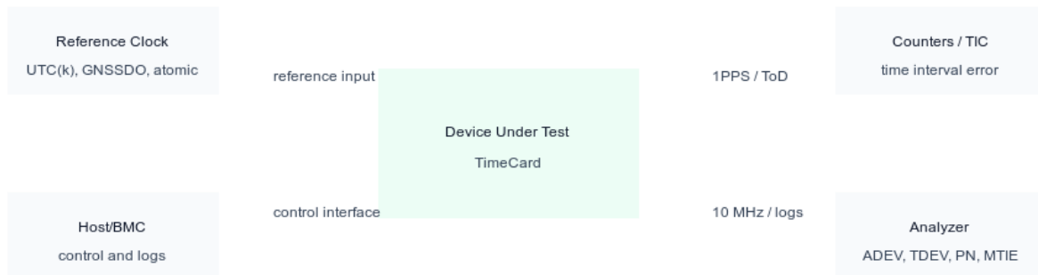
Figure 3: Figure B-1 - Representative TimeCard test fixture
