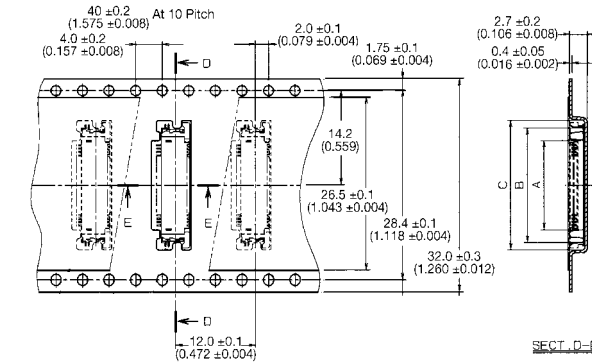
SECT. D-D
