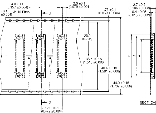
SECT. D-D
