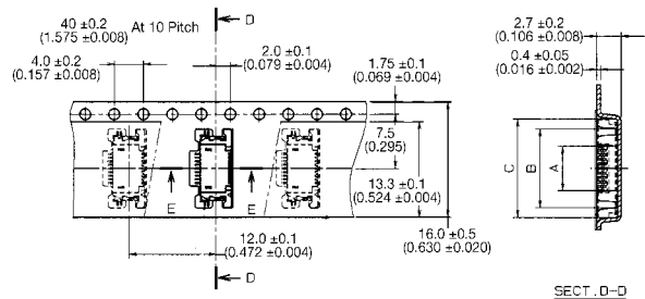
SECT. D-D
