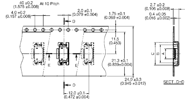
SECT. D-D
