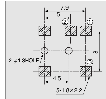
LAND LAYOUT
