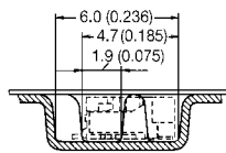
SECT. E-E
