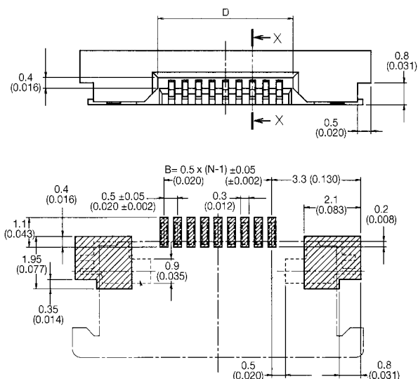
MOUNTING LAYOUT (CONN. MOUNTING SIDE)
