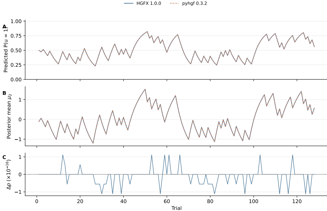
Figure 3: Perceptual trajectories agree at binary64 rounding scale, with residuals shown separately. HGFX 1.0.0 and pyhgf 0.3.2 are compared on the frozen 128-trial three-level binary-HGF cell. Panels show predicted input probability, level-2 posterior mean, and the signed HGFX-minus-pyhgf probability residual in units of 1e-16. Participant-response NLL is a separate quantity and remains not directly comparable in this cell.
