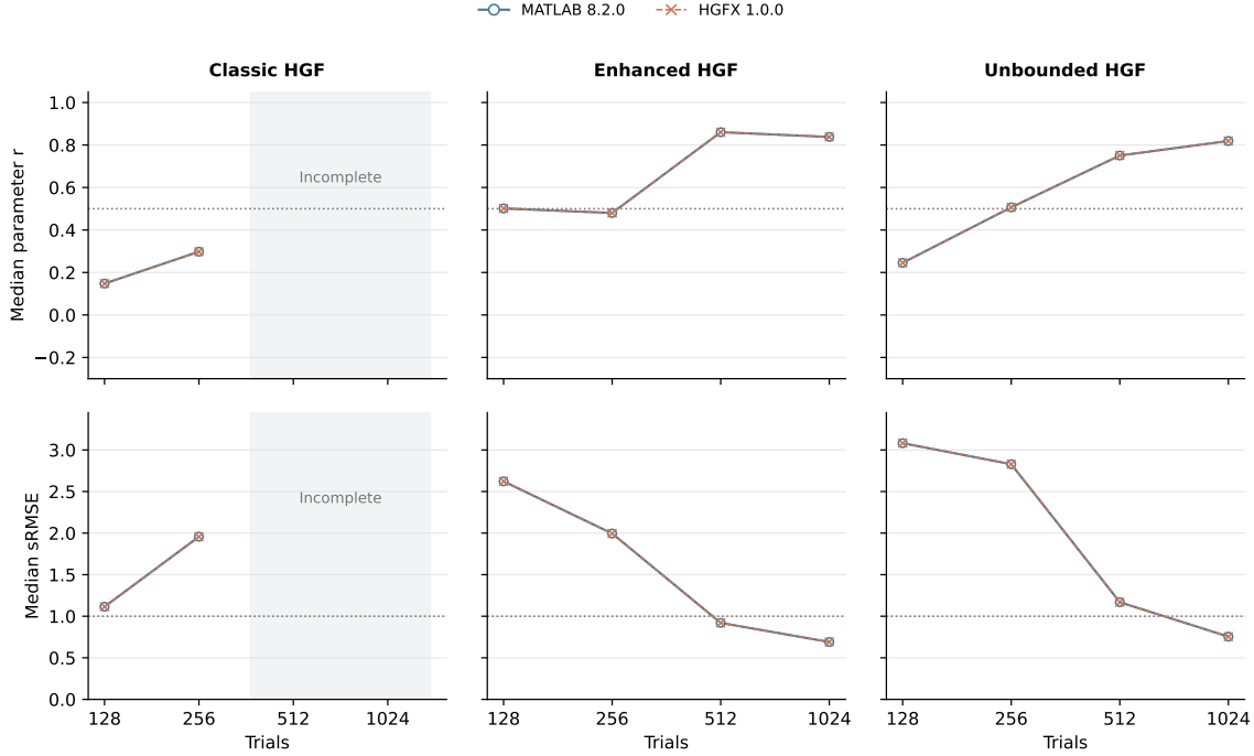
Figure 2: Trial-horizon diagnostics with incomplete cells retained. Columns separate classic, enhanced, and unbounded HGF; rows show median parameter correlation and median standardized RMSE at 128, 256, 512, and 1024 trials. Dotted lines mark the original targets. Shaded regions denote incomplete classic-HGF summaries at 512 and 1024 trials and are not zeros or interpolated estimates. The whole-study paired-integrity requirement was not satisfied, so these trends do not establish identifiability.
