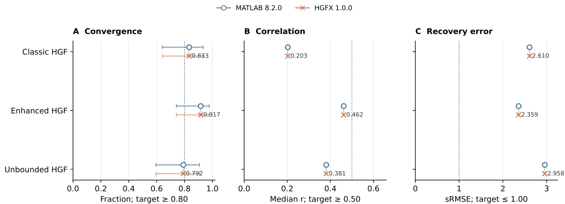
Figure 1: Close paired agreement coexists with weak recovery. Original-scale parameter-recovery summaries are shown for classic, enhanced, and unbounded HGF. Circles denote MATLAB 8.2.0 and crosses denote HGFX 1.0.0; dotted lines mark the unchanged targets. The convergence panel includes descriptive Wilson 95% intervals for 24 cases per family. Correlation and standardized-RMSE panels show point summaries because replicate-level bootstrap inputs are not available in the archived aggregate.
