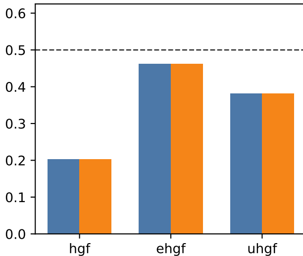
Median correlation
