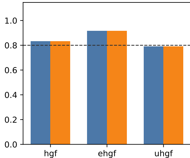
Convergence rate
