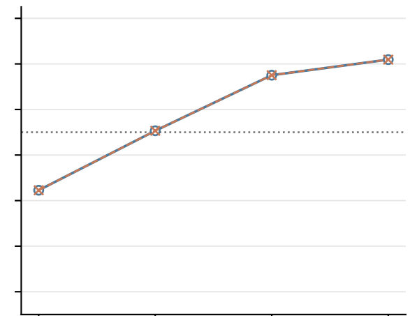
Unbounded HGF
