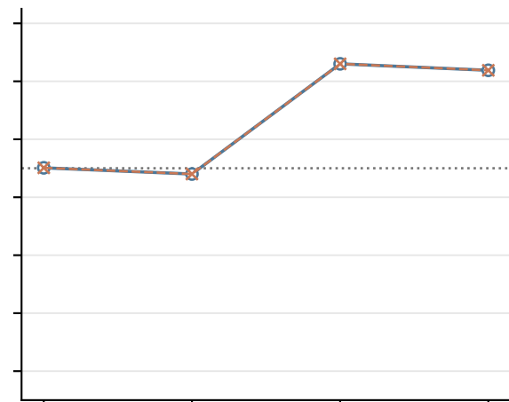
Enhanced HGF
