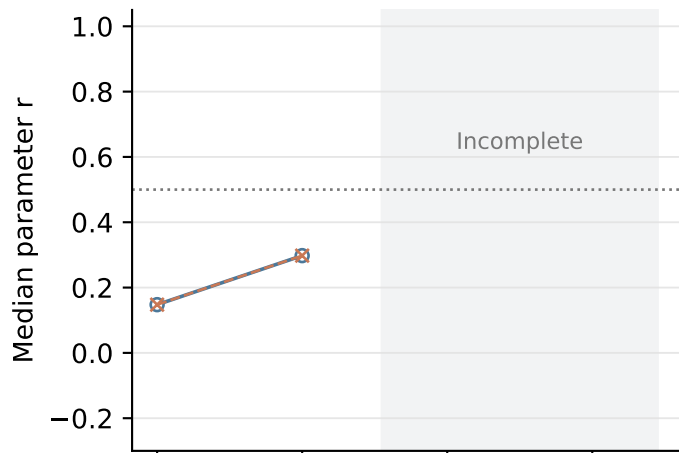
Classic HGF
