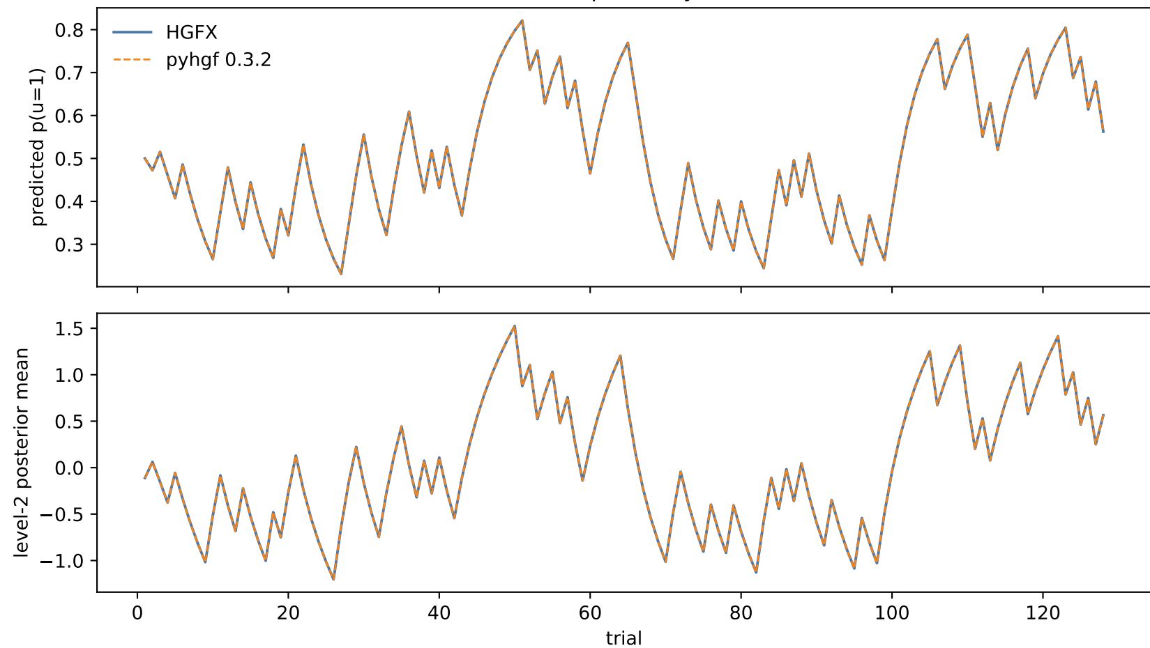
Frozen common-scope binary HGF (128 trials)
