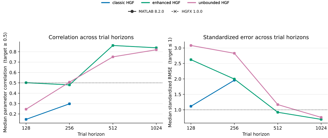
Figure 3: Prospective trial-horizon diagnostic at 128, 256, 512 and 1024 trials. MATLAB and HGFX trajectories are shown together for complete cells; incomplete classic-HGF cells remain as gaps. Because the paired-integrity requirement was not satisfied, the figure is diagnostic and does not establish a stronger identifiability conclusion.
