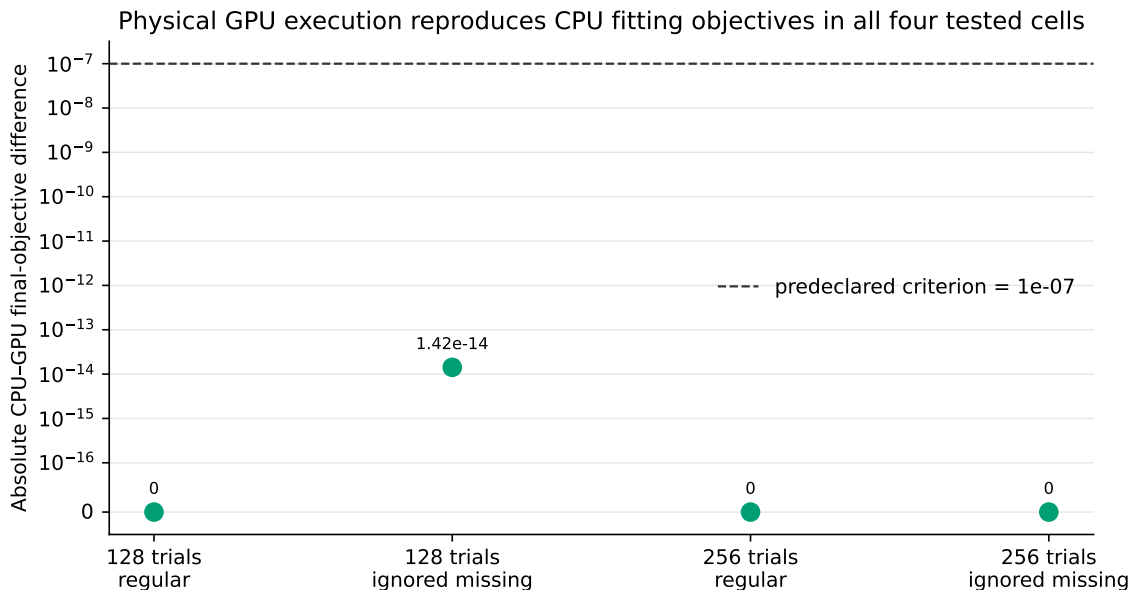
Figure 4: Absolute CPU-versus-physical-GPU final-objective differences for all four preregistered fitting cells on two Tesla T4 devices. The dashed line is the predeclared 1e-7 criterion; three cells are exactly equal at the reported precision and the maximum observed difference is 1.42e-14 . This is numerical applicability evidence, not a speed claim.
