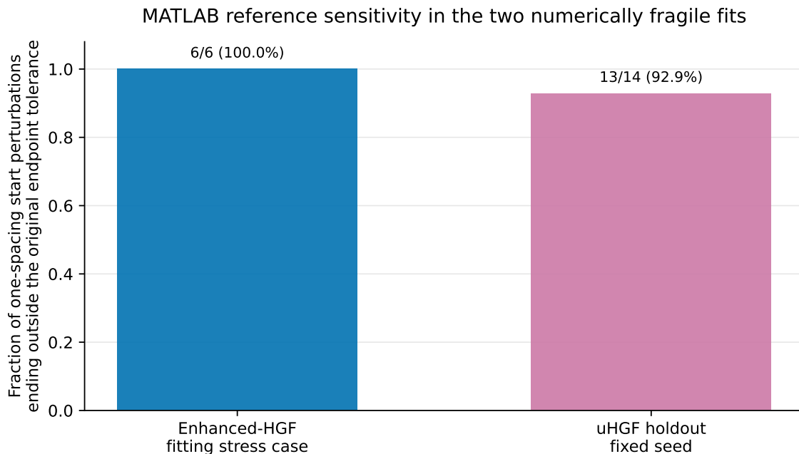
Figure 1: Sensitivity of the frozen MATLAB reference in the two numerically fragile fitting workflows. Bars show the fraction of one-local-spacing perturbations of the official start that move the MATLAB optimizer endpoint outside the original endpoint tolerance: 6/6 for the enhanced-HGF fitting stress case and 13/14 for the fixed-seed uHGF holdout. This supports an exact-scope reference-limitation interpretation without converting either endpoint mismatch into direct fitting parity.
