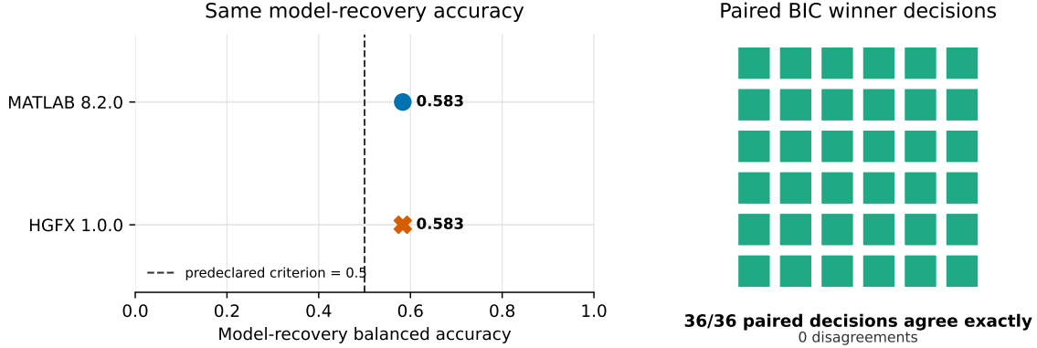
Figure 2: Paired model-selection agreement on the frozen three-model grid. MATLAB 8.2.0 and HGFX 1.0.0 have the same balanced accuracy (0.583) and identical BIC winner decisions in all 36/36 paired datasets. The dashed line marks the predeclared balanced-accuracy criterion of 0.50. Parameter-recovery metrics are reported separately in Table 4 and Supplementary Appendix S3.
