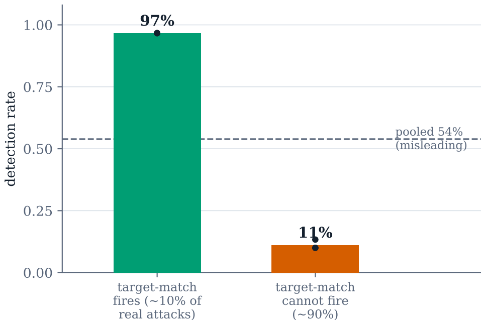
Detection on externally-authored attacks, by stratum (k=3 recordings; dots = per-run)
