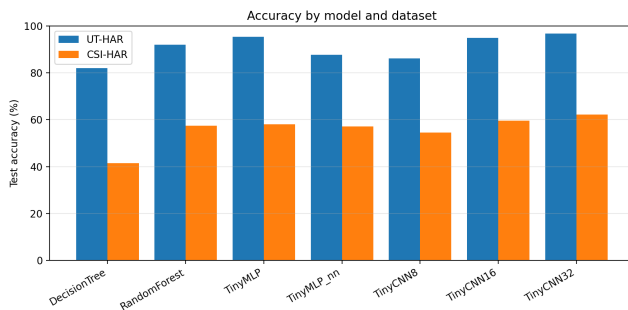
FIGURE 4. Accuracy of the classical and tiny tiers across UT-HAR and CSI-HAR. Accuracy is consistently lower on CSI-HAR, the single-ESP32 dataset with fewer samples per class.
