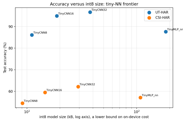
FIGURE 3. Accuracy versus int8 size for the tiny networks on both datasets (size on a logarithmic axis). The 16-channel tiny CNN sits at the top-left on both datasets, giving the best accuracy per kilobyte. The int8 file size is a lower bound on on-device cost; the runtime arena, which is what meets the device budget, is measured separately.
