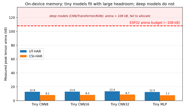
FIGURE 2. Measured peak tensor arena of the tiny networks on the classic ESP32, against the roughly 108 kB SRAM budget (dashed line). Every tiny model uses 8 to 13 kB, an order of magnitude below the budget, while the deep models exceed it and fail to allocate (shaded region). This is the central deployability result.
