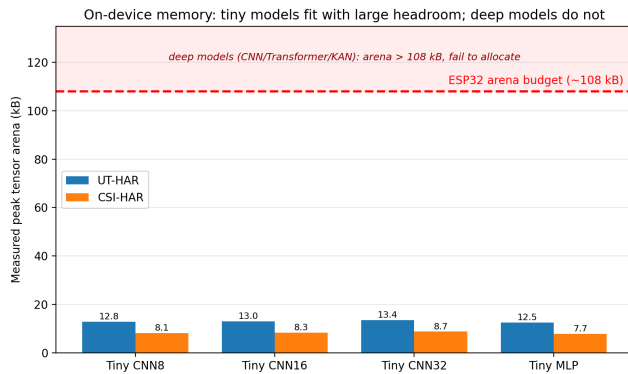
FIGURE 3. Measured peak tensor arena of the tiny networks on the classic ESP32, against the roughly 108 kB SRAM budget (dashed line). Every tiny model uses 8 to 13 kB, an order of magnitude below the budget, while the deep models exceed it and fail to allocate (shaded region). This is the central deployability result.
