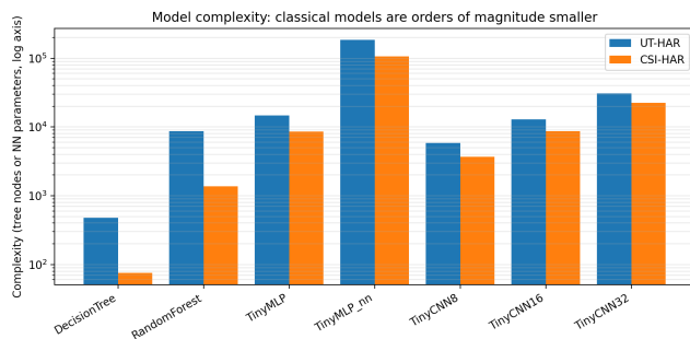
FIGURE 6. Model complexity on a logarithmic axis (tree node count or network parameter count). The classical learners are one to three orders of magnitude smaller than the networks, which is why they fit the device with large margins.
