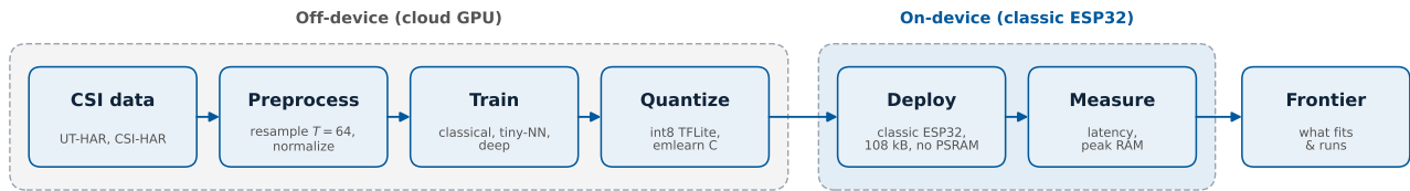
FIGURE 1. System and measurement pipeline. Models are trained and quantized off-device on a cloud GPU, then exported as int8 TensorFlow Lite (neural models) or emlearn C (classical models), deployed on the bare classic ESP32, and measured for on-device latency and peak RAM. The two deployment walls, convertibility and memory, are evaluated at the deploy stage, and the result is the deployability frontier.
