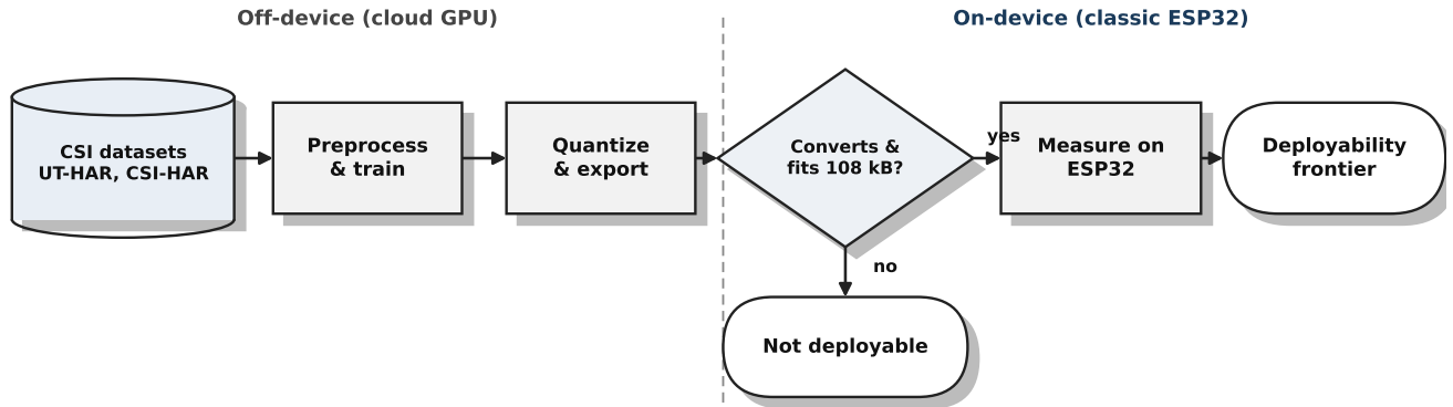
FIGURE 1. System and measurement pipeline. Models are trained and quantized off-device on a cloud GPU, then exported as int8 TensorFlow Lite (neural models) or emlearn C (classical models), deployed on the bare classic ESP32, and measured for on-device latency and peak RAM. The two deployment walls, convertibility and memory, are evaluated at the deploy stage, and the result is the deployability frontier.
