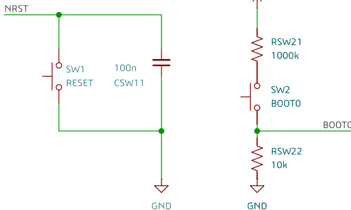
RESET AND BOOT
