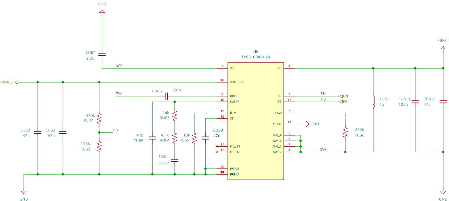
TPS61088 BOOST 3A 6V
