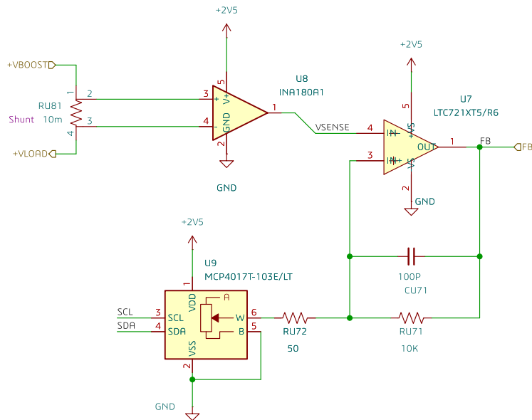
HIGH SIDE CURRENT SEMSE
