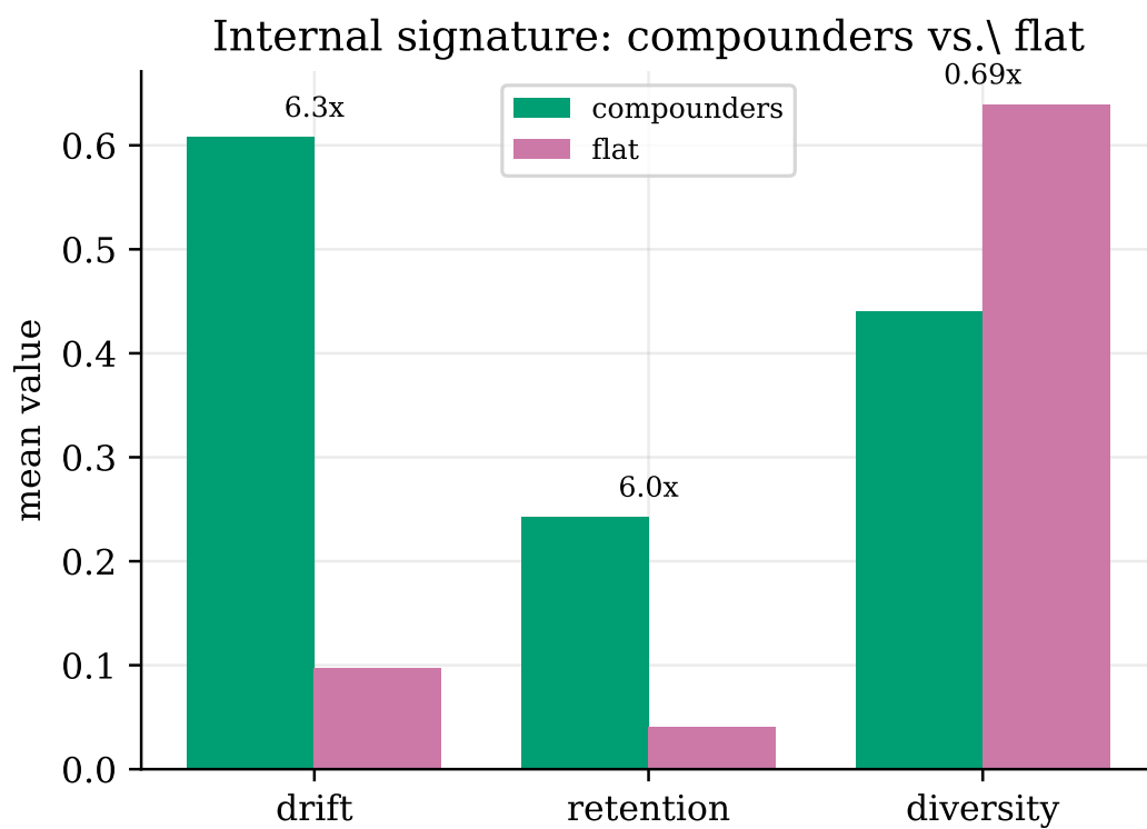
Figure 3: The internal signature that separates compounders from flat runs among wall-crossers: sustained drift and retention are \sim 5\text{--}6\times higher in compounders, while generation diversity is lower (productive convergence, not diversity preservation).
