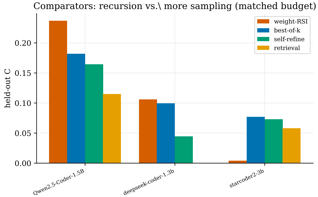
Figure 16: Is it really recursion? Weight-RSI vs. non-recursive controls (best-of-k, self-refine, retrieval) at matched generation budget. \text{recursion\_gain} = \text{weight-RSI} - \text{best comparator} .
