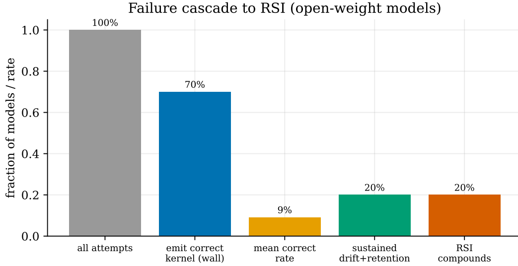
Figure 20: Attrition from attempt to compounding RSI across open-weight models: most attrition happens at the correctness wall (emitting any correct kernel) and again at sustained plasticity+retention.
