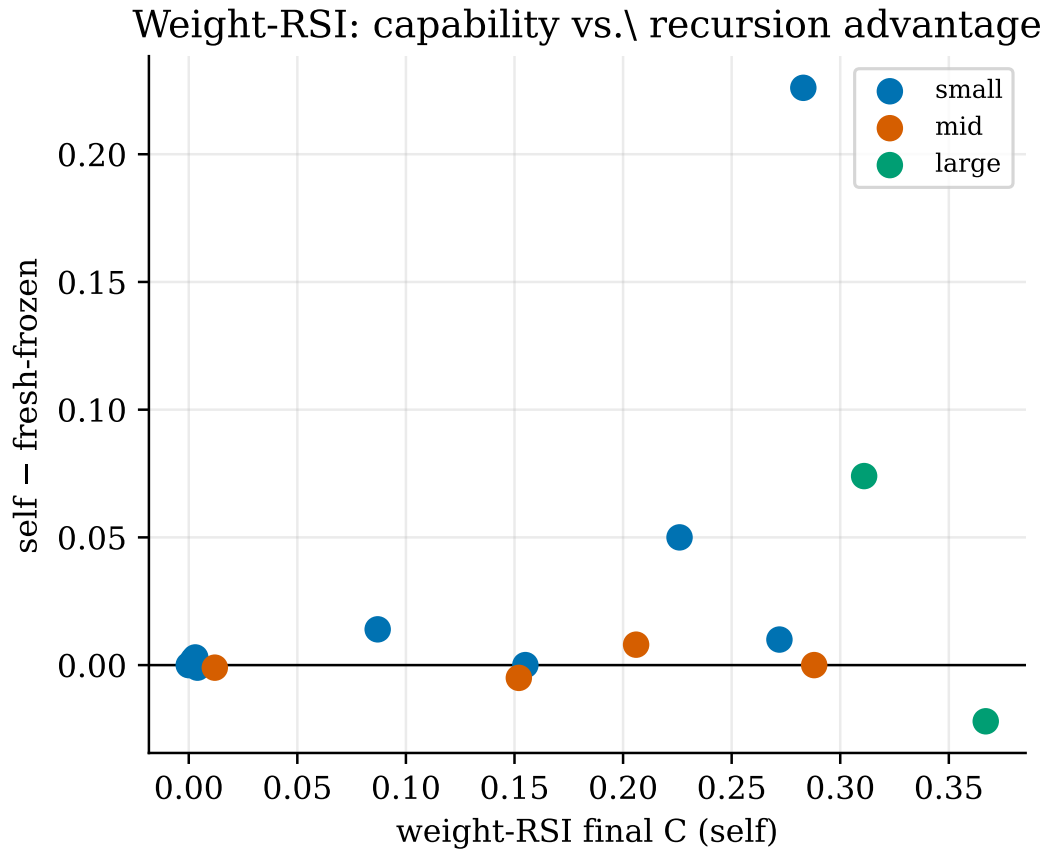
Figure 17: Weight-RSI: final self-trained held-out C vs. the self-minus-fresh-frozen advantage (positive = training on own kernels beats an equal-budget fresh baseline).
