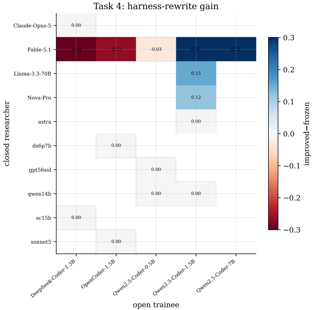
Figure 13: Task 4 (closed→open): a closed frontier researcher rewrites an open trainee’s training harness. Cell = improved - frozen held-out C on the trainee (positive = the rewritten harness helps).
