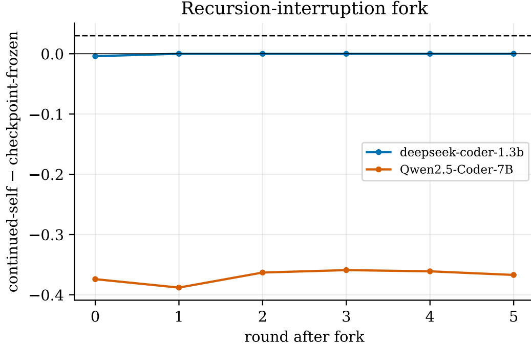
Figure 18: Recursion-interruption control: continued self-training vs. a checkpoint-frozen producer at equal budget. Sustained > 0 = genuine compounding rather than a one-time producer upgrade.
