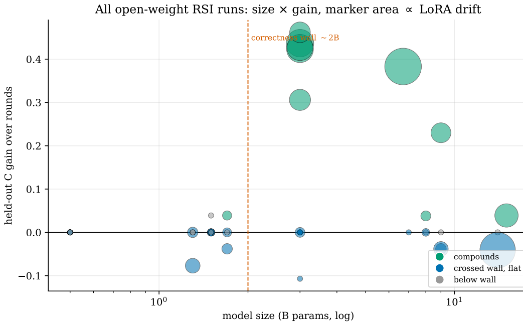
Figure 21: Every open-weight weight-RSI run positioned by model size ( x ) and held-out C gain ( y ); marker area \propto sustained LoRA drift; color = outcome. The 2B correctness wall and the mid-scale compounding band are visible at a glance.
