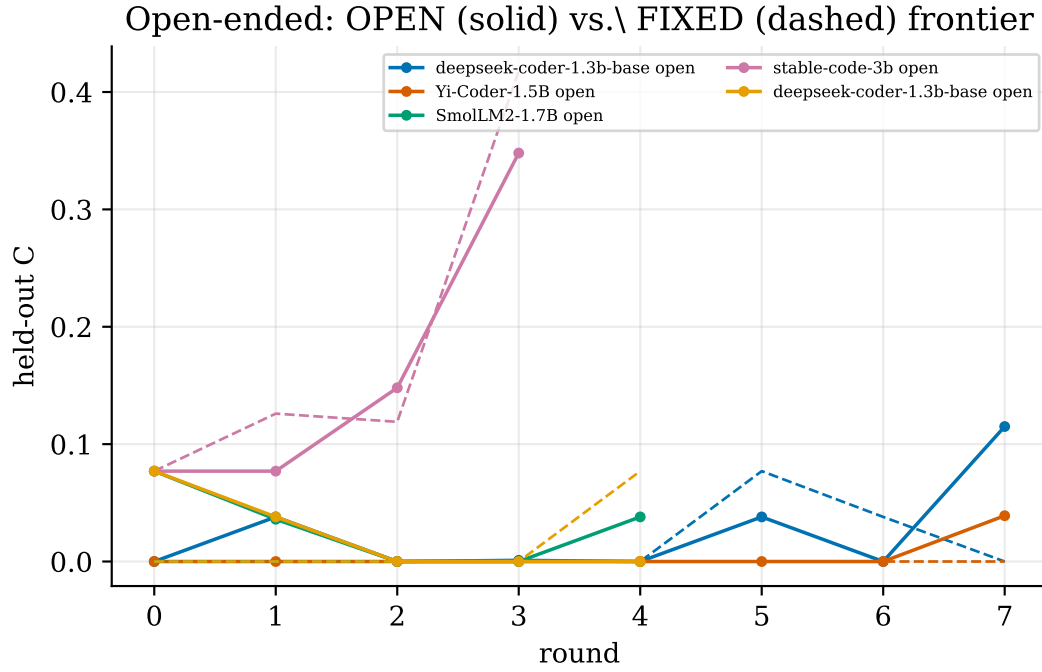
Figure 12: Open-ended RSI: a learner facing an OPEN escalating self-authored frontier (solid) vs. a FIXED static frontier (dashed) at equal budget. Overlap means open-endedness is a one-time upgrade, not compounding.
