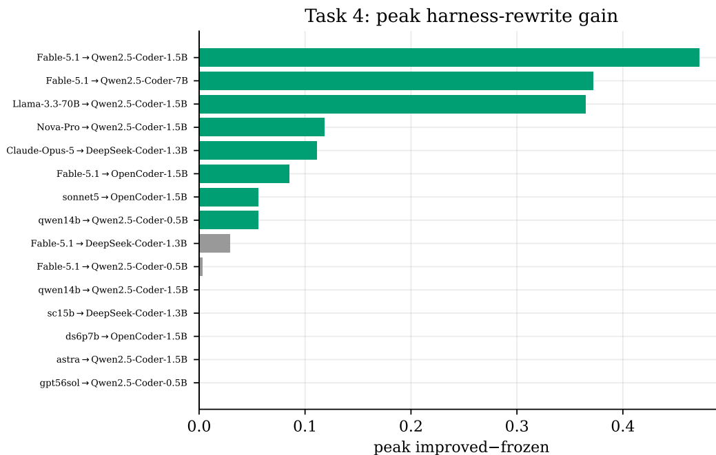
Figure 14: Peak improved-frozen over rounds for each researcher→trainee pair.
