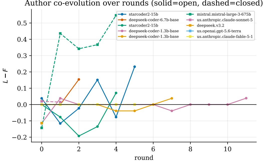
Figure 10: Per-round L-F trajectories (solid = open-weight, dashed = closed/API). Long horizons reveal whether early positive spikes compound or regress to zero.
