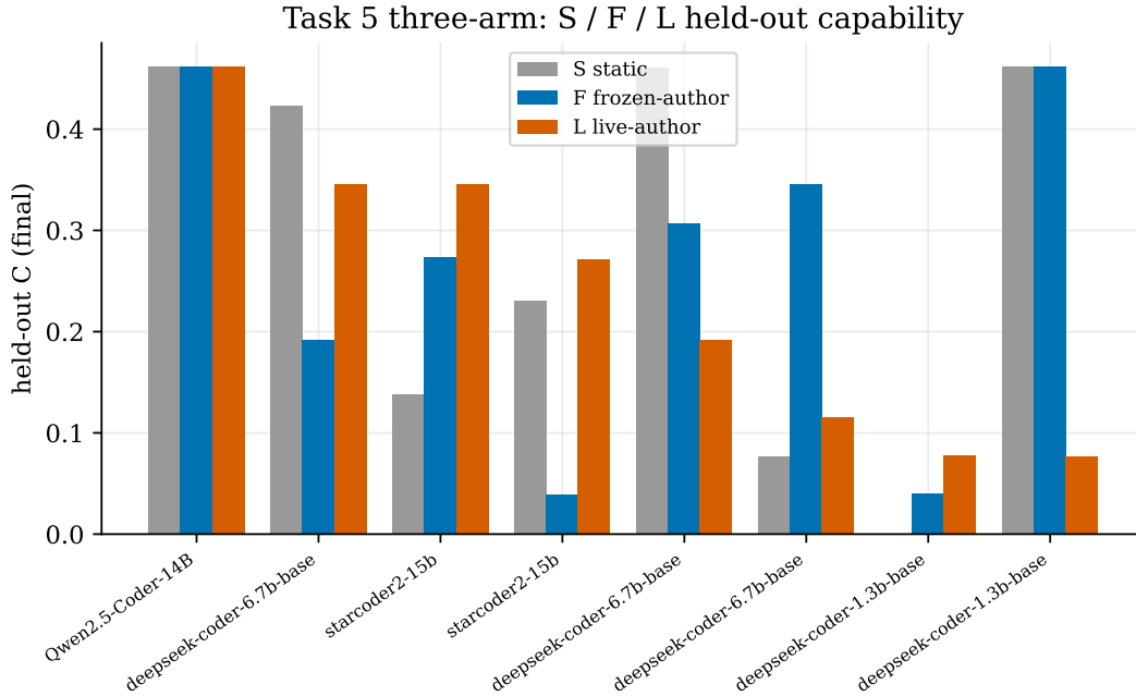
Figure 9: Three-arm self-play at equal budget on a fixed held-out ladder: STATIC (fixed frontier), FROZEN-AUTHOR (escalating frontier, frozen base author), LIVE-AUTHOR (co-evolving author). F - S isolates the adaptive-curriculum benefit; L - F isolates author co-evolution.
