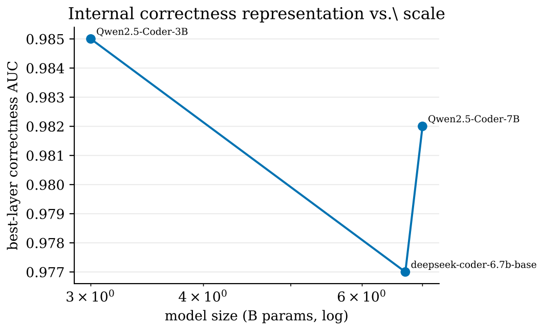
Figure 6: Best-layer correctness-decodability AUC vs. model scale. (Populated as more interpretability probes land.)
