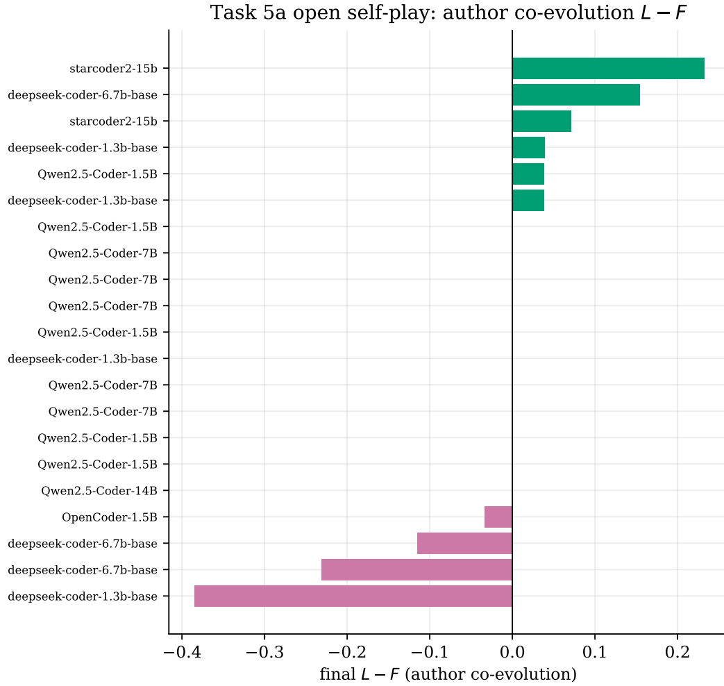
Figure 7: Final L - F (live-author minus frozen-author, the self-referential signal) per open-weight model. > 0 means updating the author beyond a frozen-author escalating curriculum genuinely helps.
