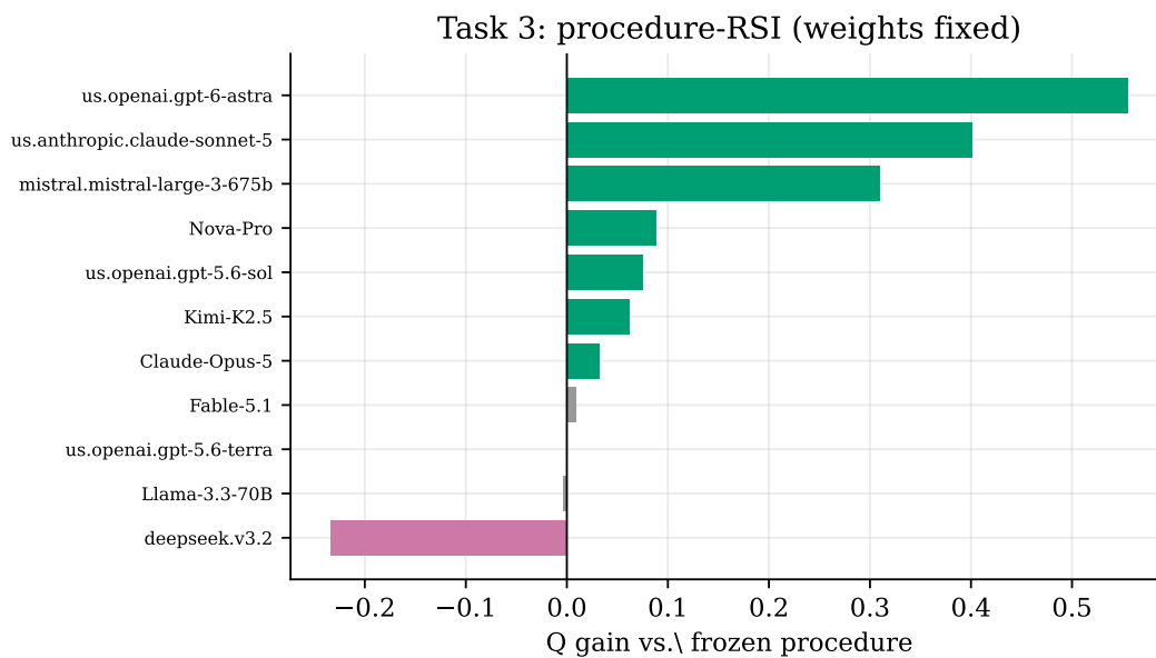
Figure 15: Task 3: a frozen-weight model rewrites its own strategy library + verified archive. Held-out Q gain vs. the frozen procedure; frontier models improve their own procedure substantially.
