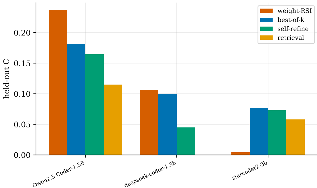
Comparators: recursion vs.\ more sampling (matched budget)
