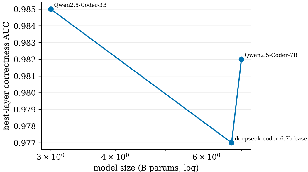
Internal correctness representation vs. \ scale
