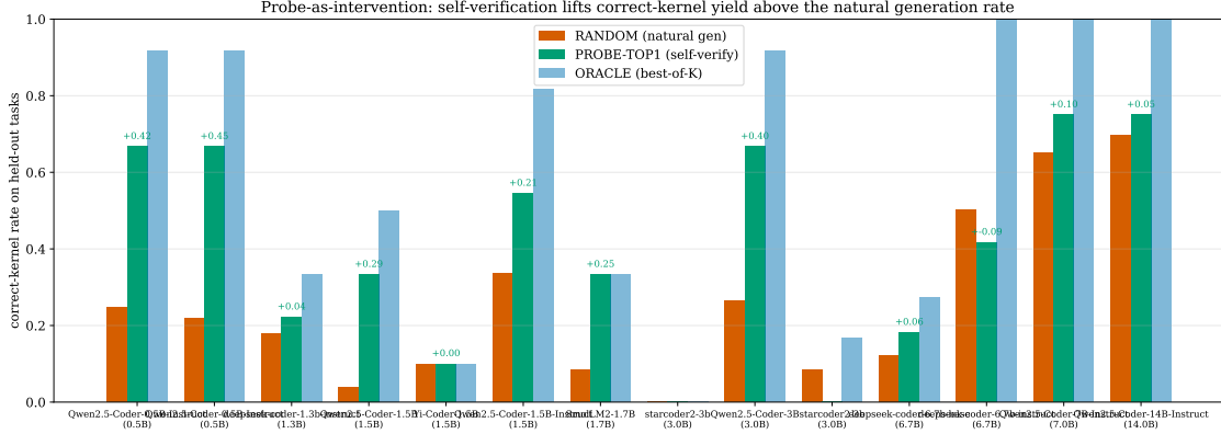
Figure 40: Self-verification (probe-guided selection) vs. the model’s natural single-draw success (RANDOM) and the ORACLE best-of- K upper bound, at equal generation budget K , on held-out tasks. Annotated +lift = PROBE-TOP1 - RANDOM . Probe selection recovering much of the oracle gap turns the correlational correctness-AUC into a causal decode-time intervention.
