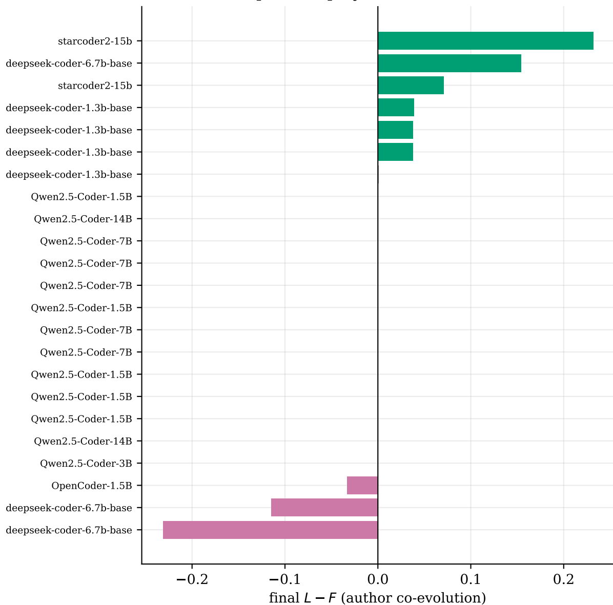
Task 5a open self-play: author co-evolution L - F
