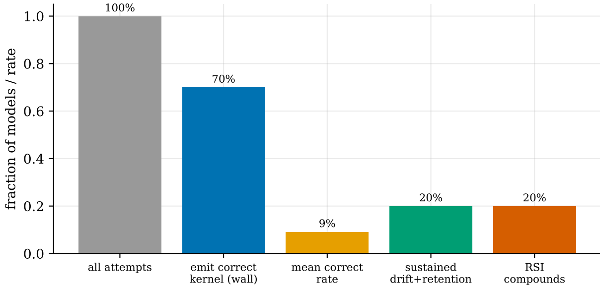
Failure cascade to RSI (open-weight models)
