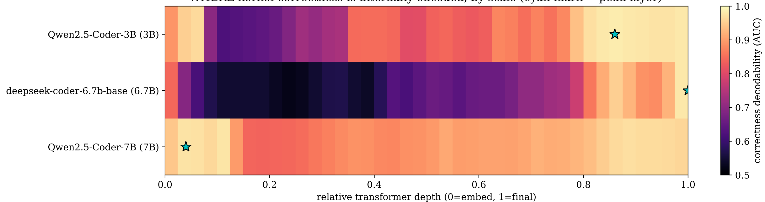
WHERE kernel-correctness is internally encoded, by scale (cyan mark = peak layer)
