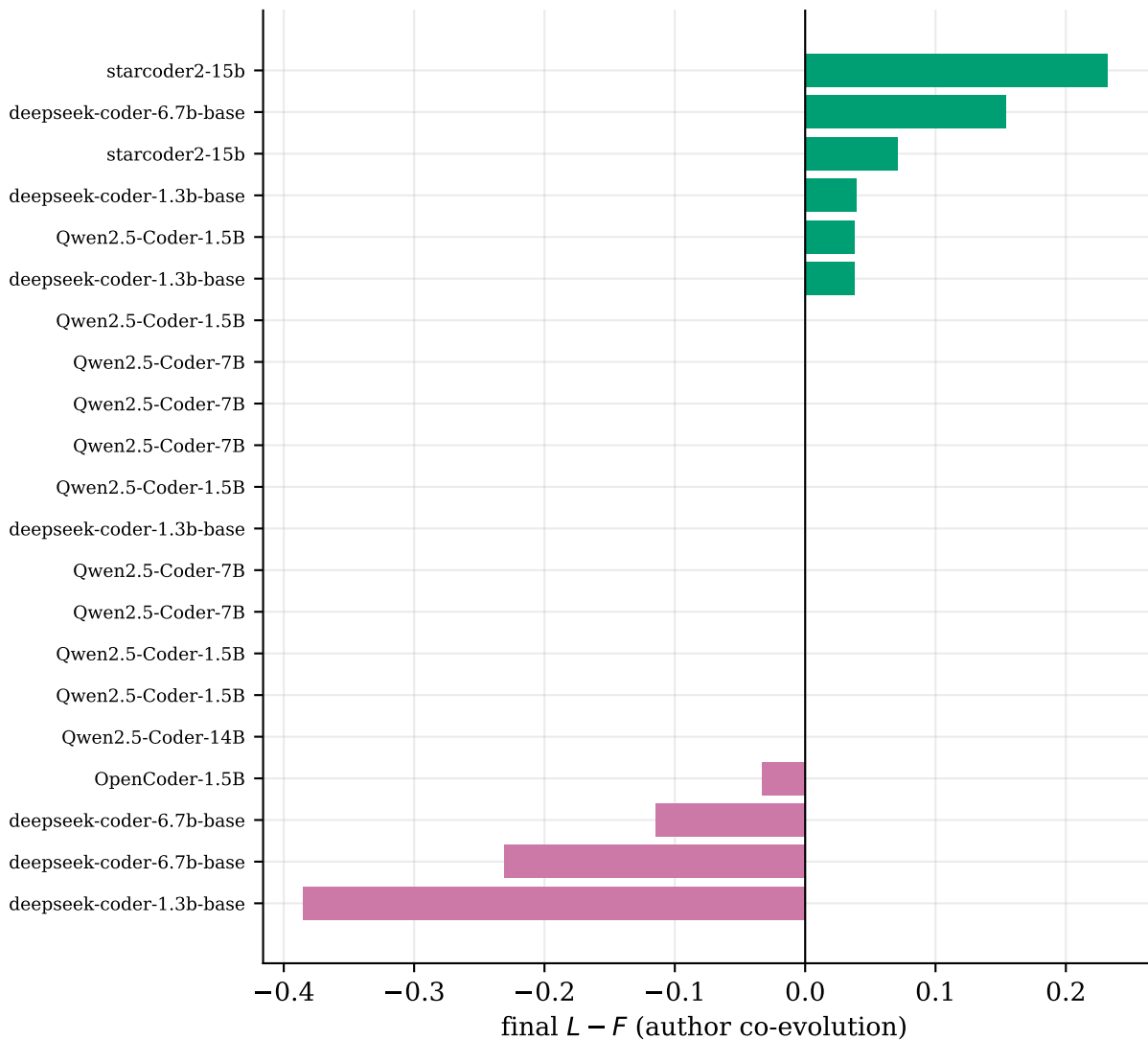
Task 5a open self-play: author co-evolution L - F
