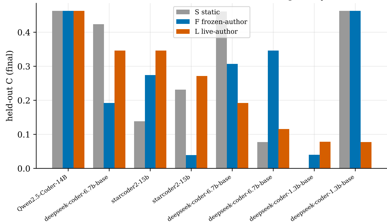
Task 5 three-arm: S / F / L held-out capability
