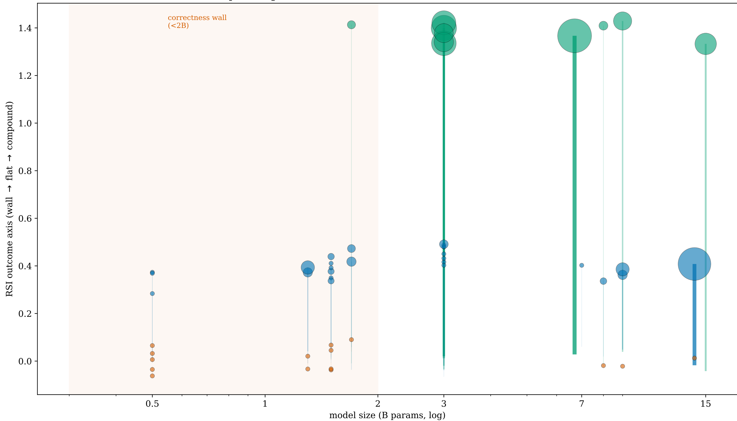
All 50 open-weight runs: size vs.\ outcome, marker area & lift \propto LoRA drift
